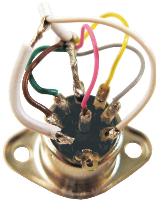
Powerlink connections.
